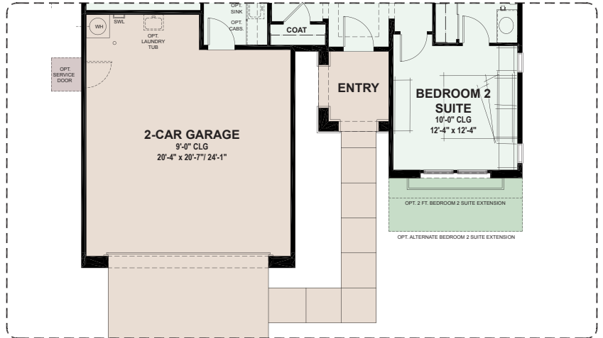
Elevation C
