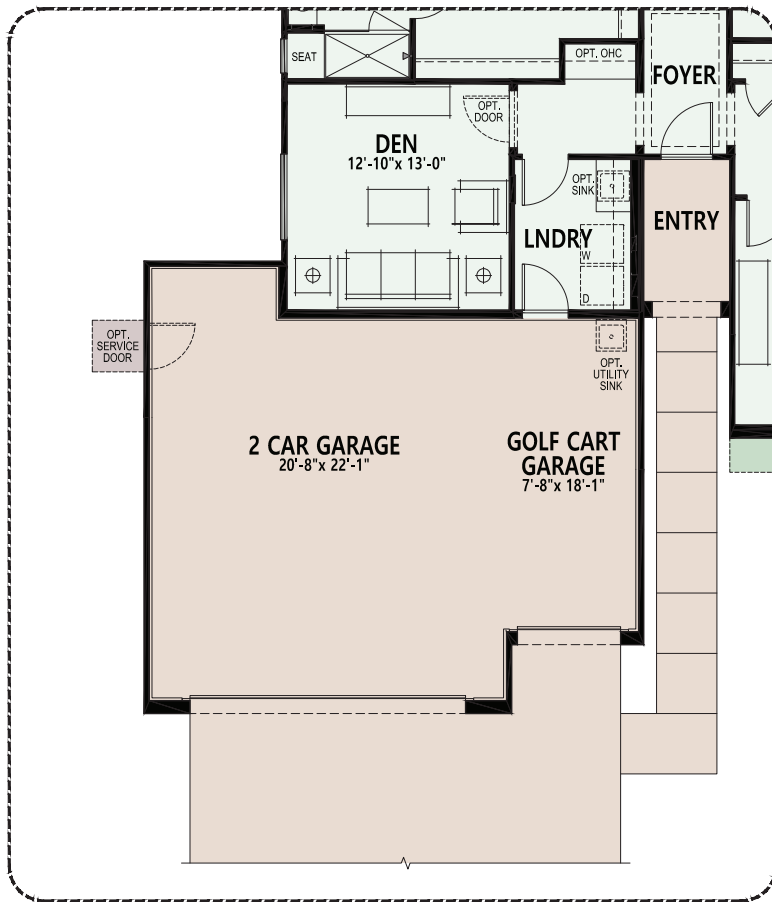
Opt. 3 ft Expanded Den w/ Opt. Expanded Laundry w/ Opt. 4 ft Garage Extension at Opt. Golf Cart Garage
