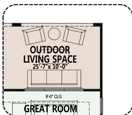
Opt. Privacy Wall
