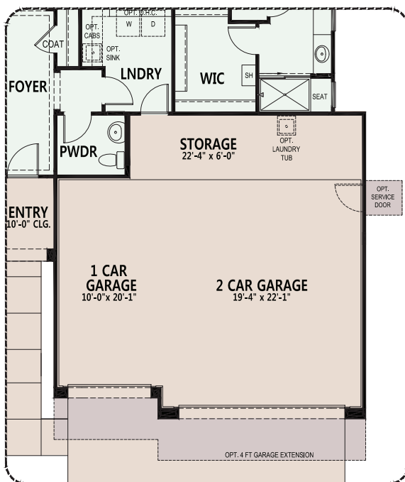
Opt. 3 Car Garage
